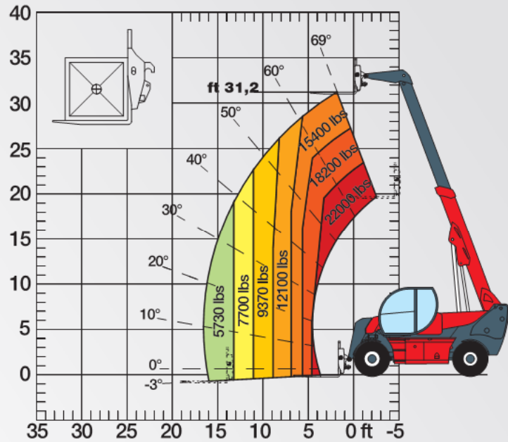
Load chart with forks
